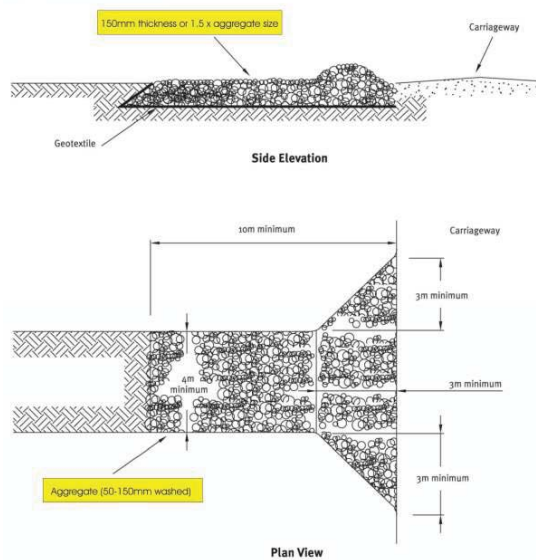
Figure 1.8 Stabilised Construction Entrance
