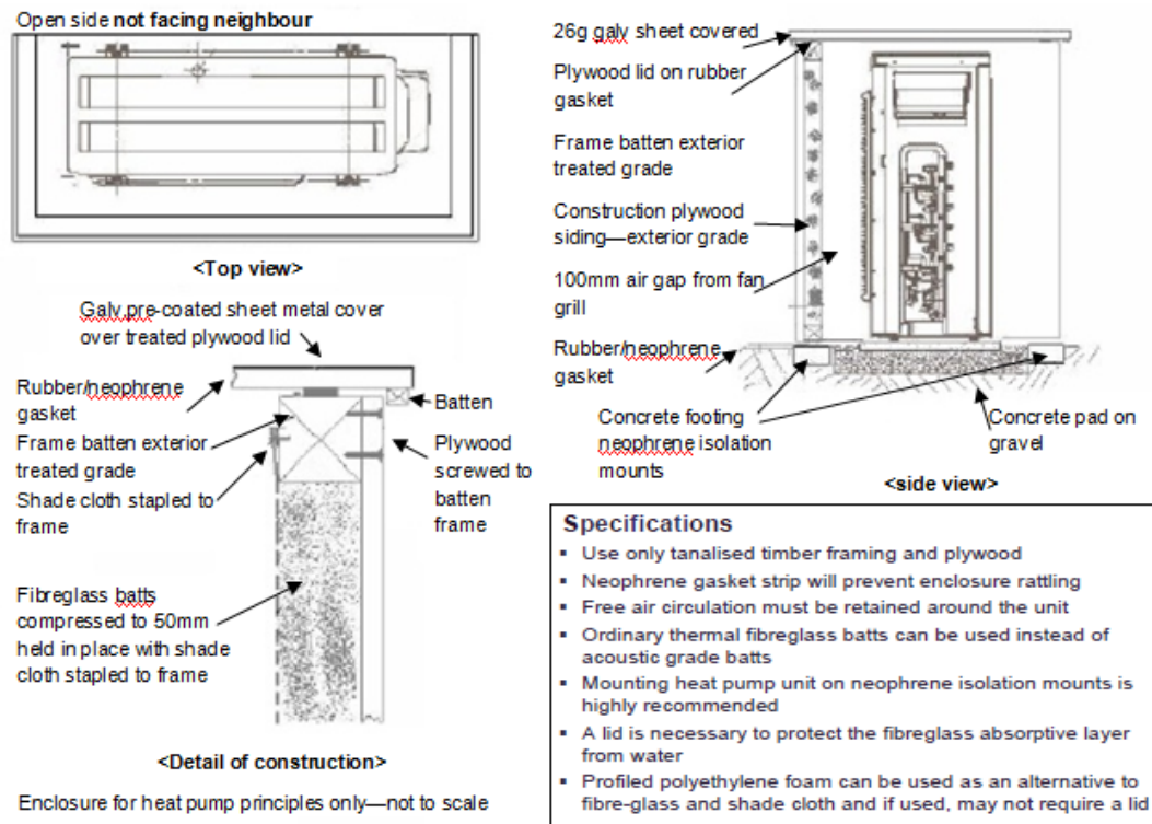
Figure 4 – a three-sided heat pump enclosure
