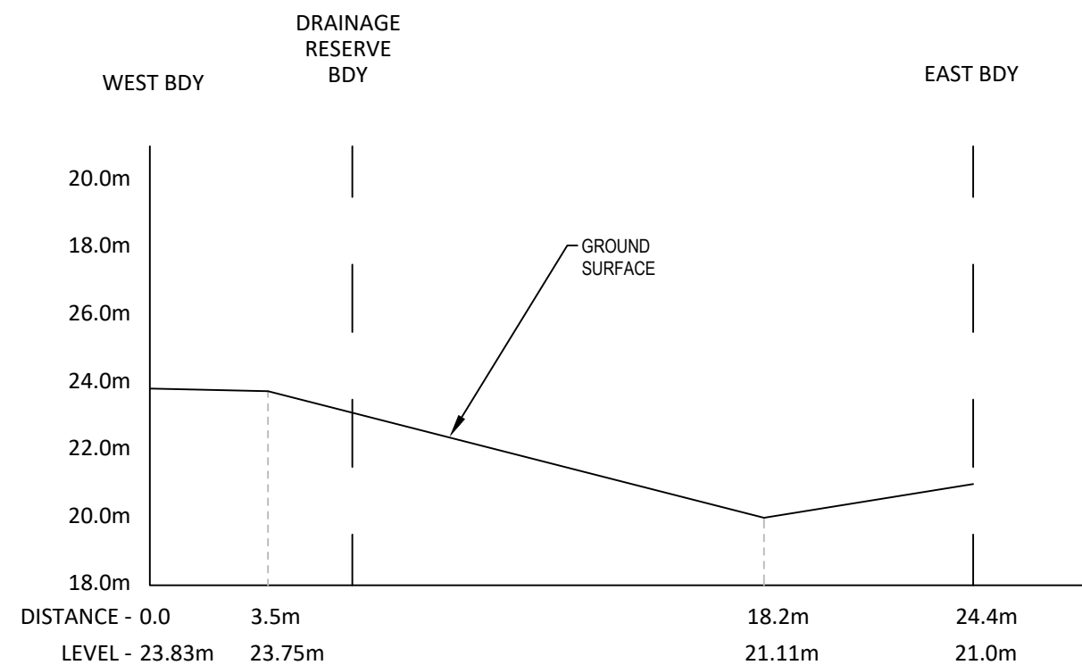
FRONT BDY CROSS-SECTION 1-1 (SCALE 1:200 NATURAL)
