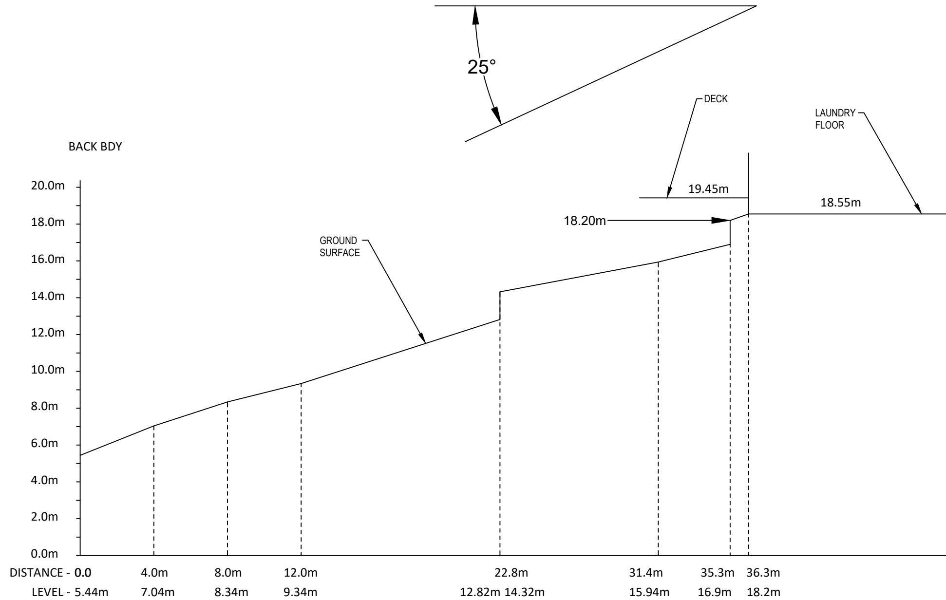
GULLY LONG SECTION (SCALE 1:200 NATURAL)
