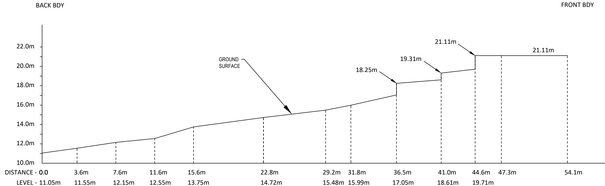
EAST BOUNDARY LONGSECTION (SCALE 1:200 NATURAL)
