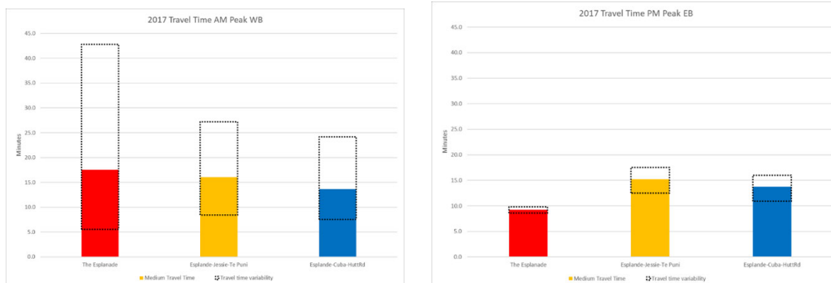
Figure 13 Median Travel Times and Travel Time Variabilities (AM Peak WB on the left and PM Peak EB on the right)
